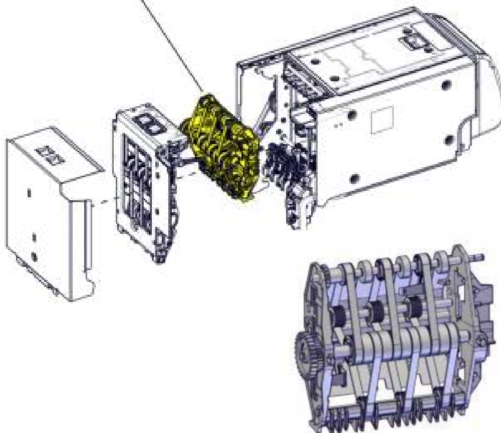
MMA HI INNER CHASSIS ASSEMBLY
