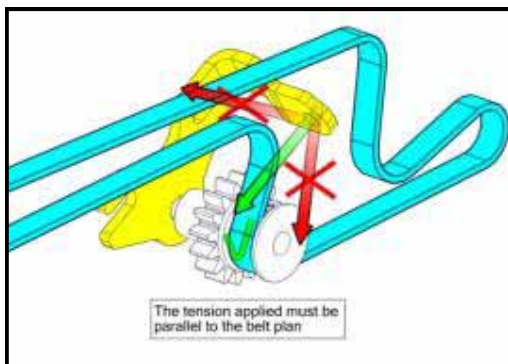
Belt tension: side view
