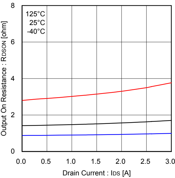
Figure 19. Output MOSFET ON Resistance
