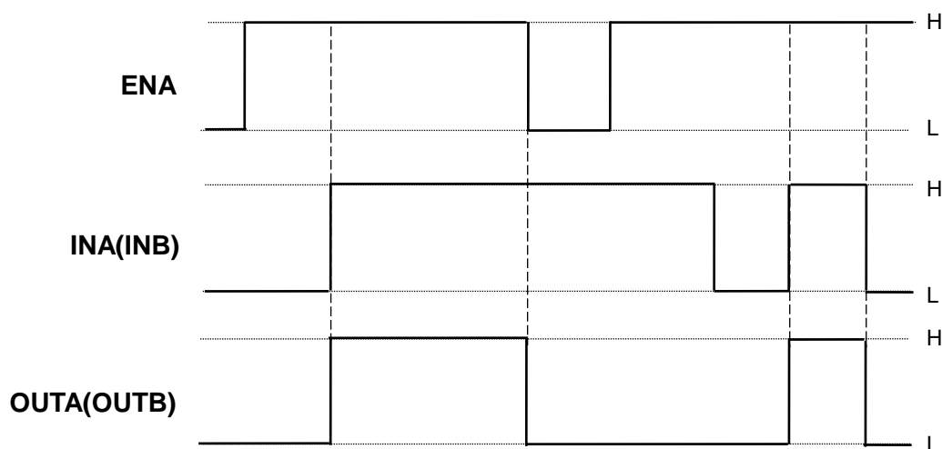
Figure 3. Input and Output Logic Timing Chart
