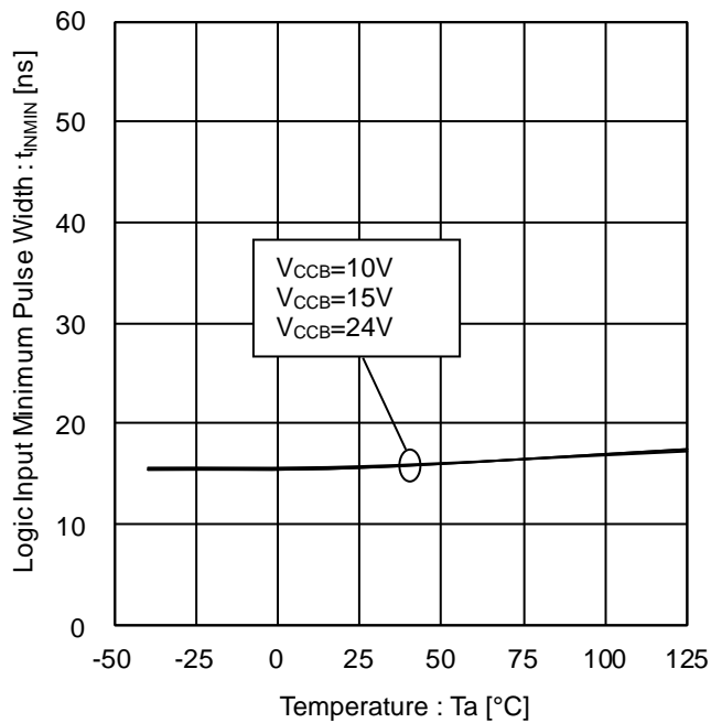
Figure 20. Logic Input Minimum Pulse Width vs Temperature
