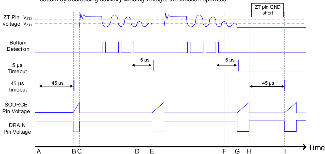
Figure 10. ZT Timeout Function
