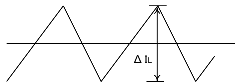
Figure 31. Inductor Current
