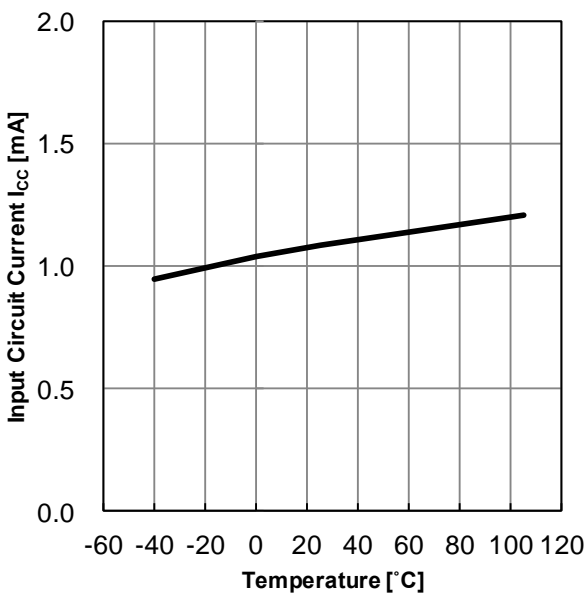
Figure 13. Input Circuit Current vs Temperature ( V_{FB}= 1.2V )
