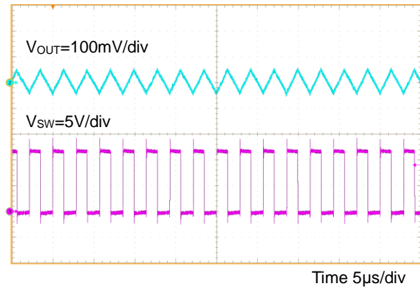
Figure 15. V_{OUT} Ripple ( V_{IN} = 12\text{V} , I_{OUT} = 1.5\text{A} )
