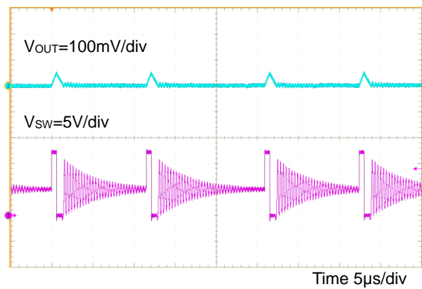
Figure 14. V_{OUT} Ripple ( V_{IN} = 12\text{V} , I_{OUT} = 10\text{mA} )
