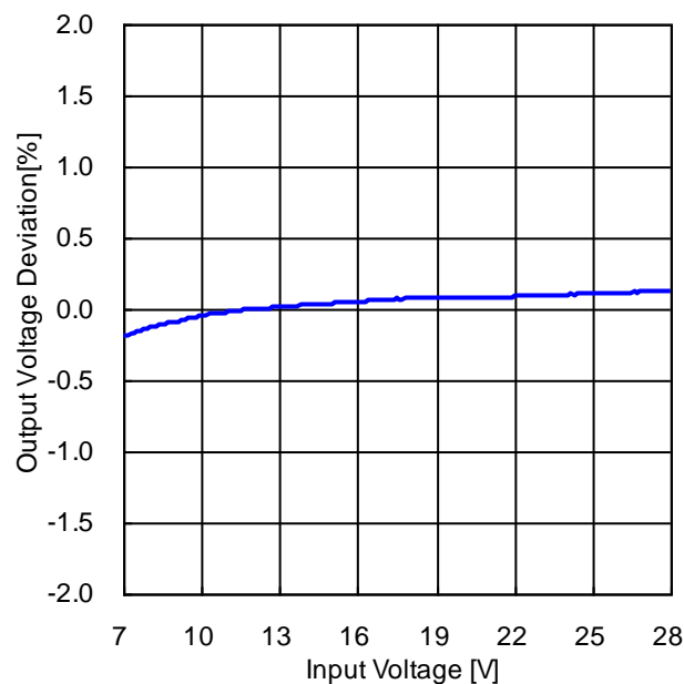
Figure 17. Line Regulation ( I_{OUT} = 1.5\text{A} )
