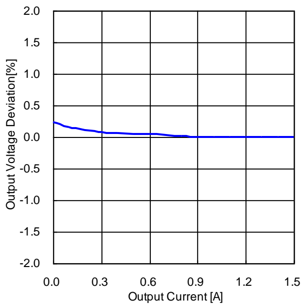
Figure 16. Load Regulation ( V_{IN} = 12\text{V} )
