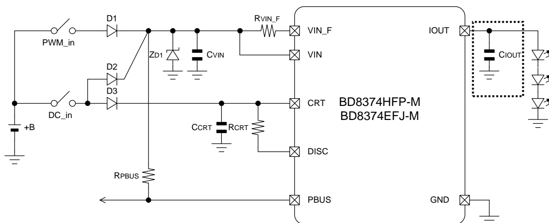
Figure 20. About the capacitor of connecting IOUT terminal
