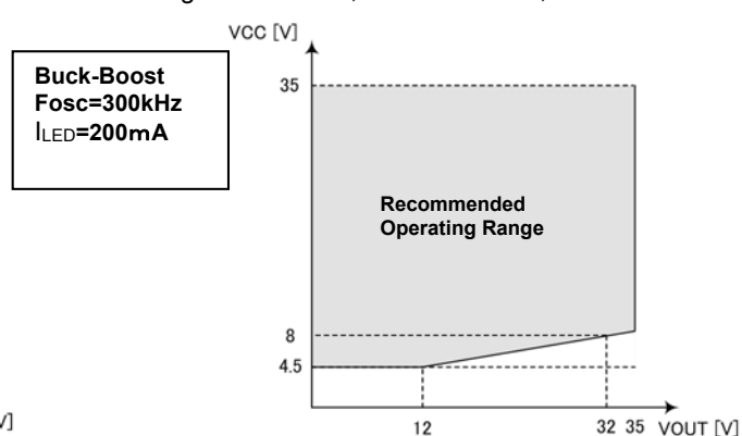
Figure 34. Buck-Boost, Fosc=300kHz, I_{LED}=200mA
