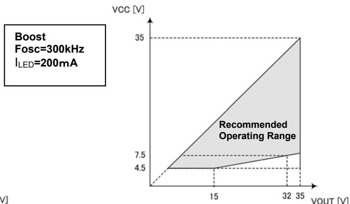
Figure 30. Boost, Fosc=300kHz, I_{LED}=200mA
