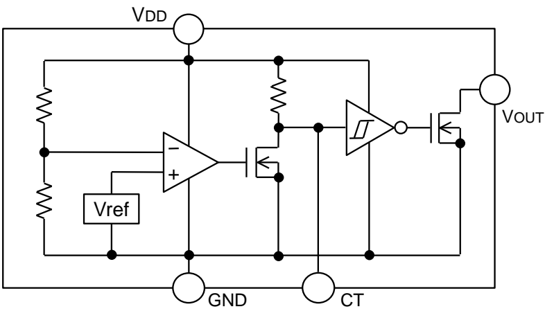
Fig.1 BD52xx Series
