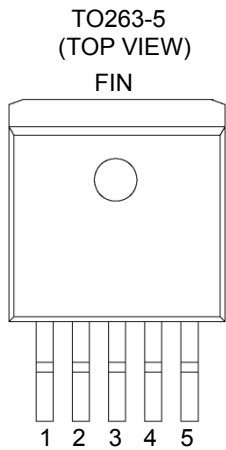
Figure 3. Pin Configuration
