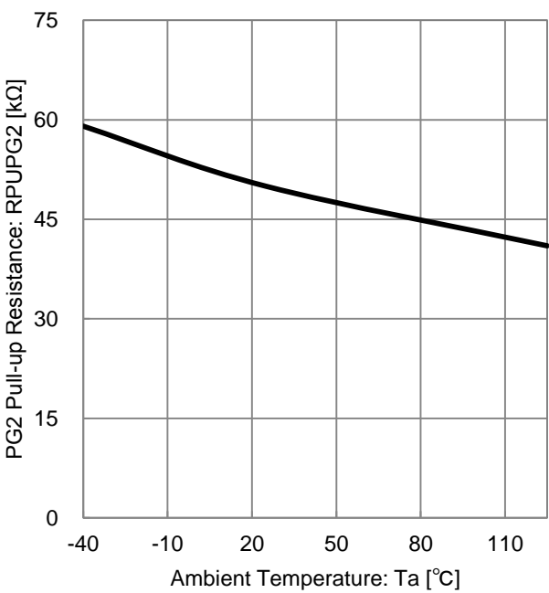
Figure 27. PG2 Pull-up Resistance vs Ambient Temperature (PG2 Pull-up Resistance)
