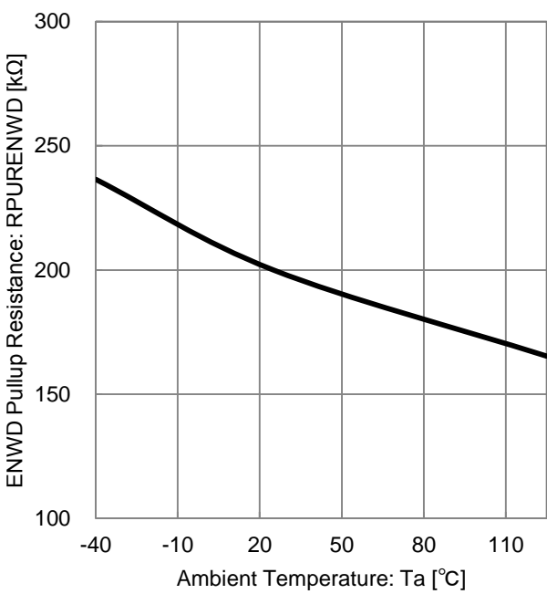
Figure 35. ENWD Pull-up Resistance vs Ambient Temperature (ENWD Pull-up Resistance)
