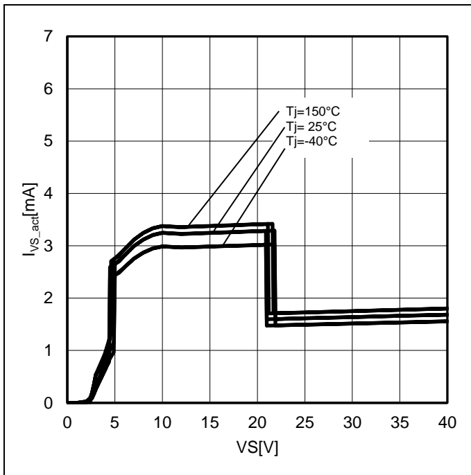
Figure 5. I_{V_S\_act} vs V_S ( Normal State ) (RSTB=VCC, SH1=SH2=PGND, Enable Register[2:0]=111, CUR_SOURCE[4:0]=00000, CUR_SINK[4:0]=00000, Protection Mode Setting[7:0]=00000000 Other address data is default value)
