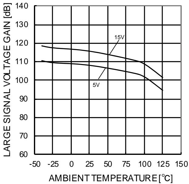
Figure 70. Large Signal Voltage Gain - Ambient Temperature ( R_L=2k\Omega )
