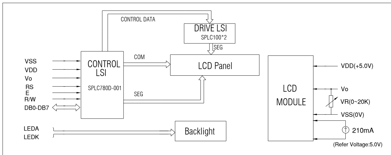
Figure 2. Block diagram
