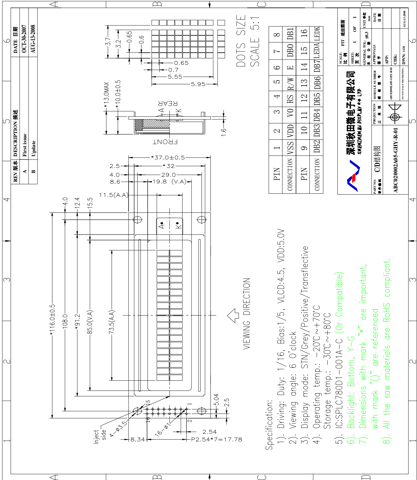
Figure 1. Dimensional outline
