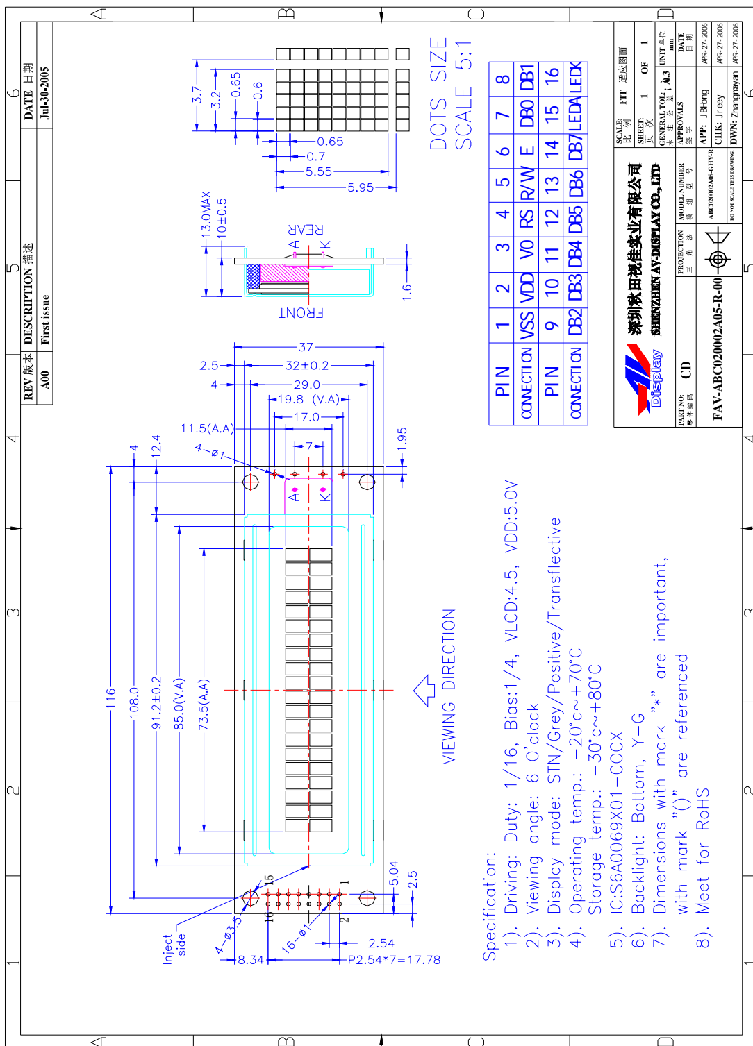
Figure 2. Dimensional outline
