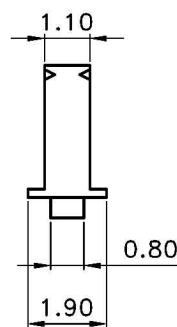
C-C SEC
