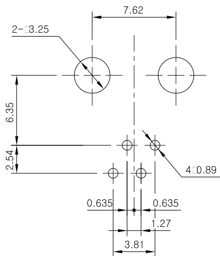
PCB LAYOUT (3/1)
