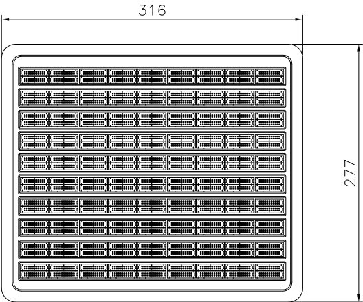
TRAY LAYOUT 902-2316R
