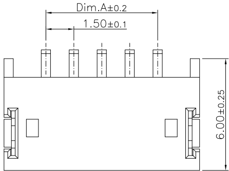
Dimension Information:
